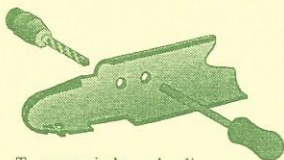
To open windows, landing gear bays, etc. drill initial hole then file or cut to shape.
